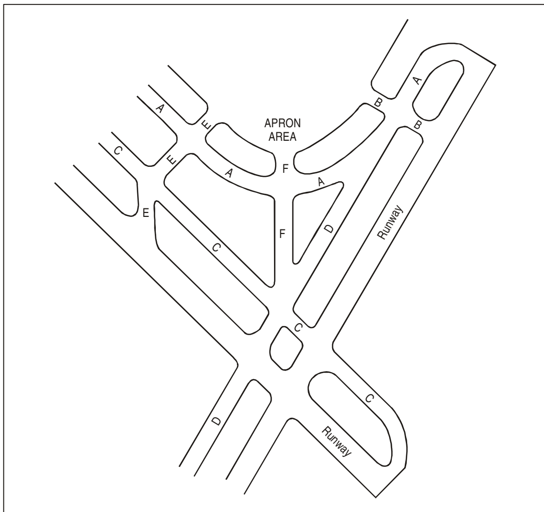
Figure 11-6. Assignment of letters to taxiways
