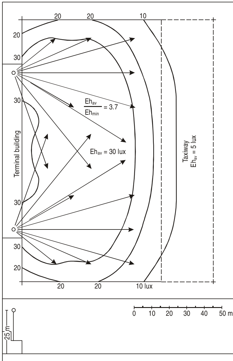
Figure 13-1. Typical isolux curves for horizontal illuminance (Example A)
