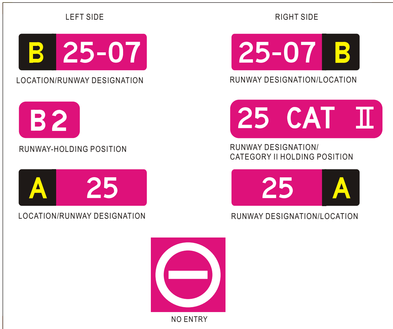
Figure 11-2. Mandatory instruction signs
