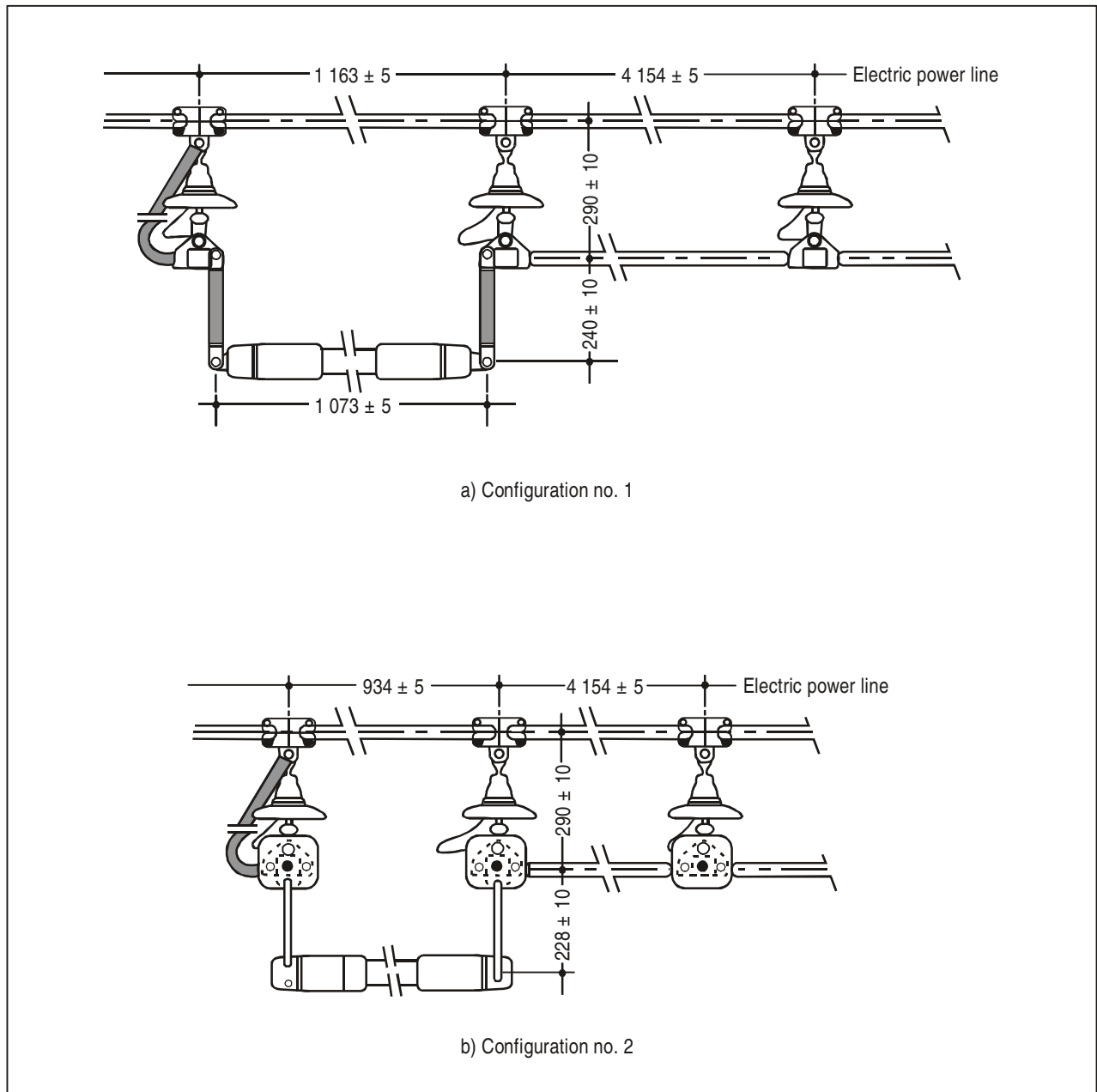
Figure 14-5. Installation of obstacle lights on high-tension wires
