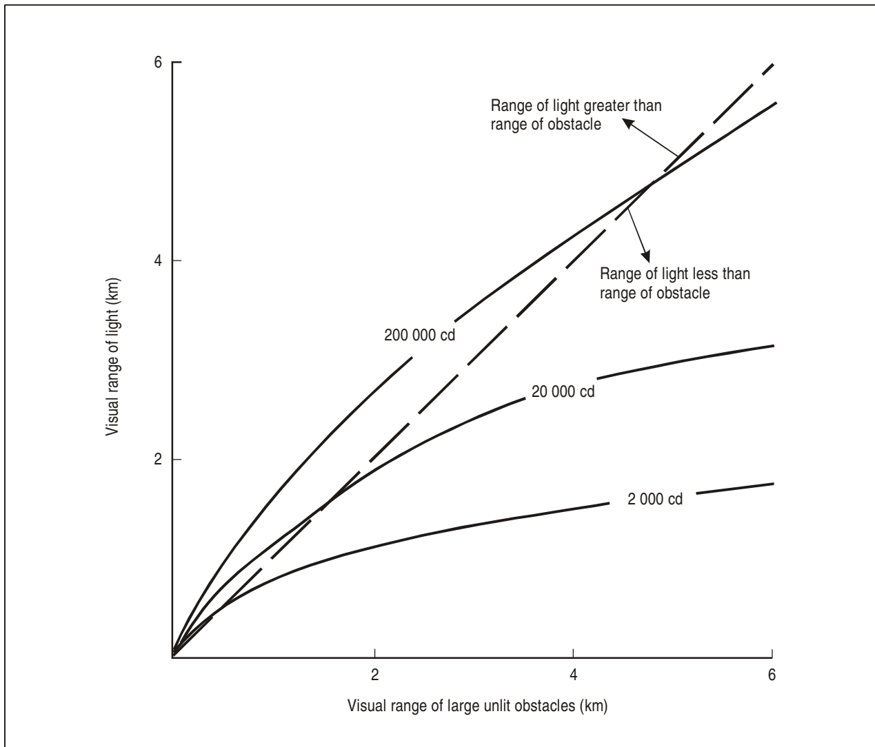
Figure 14-1. Comparison of the typical daytime range of lights and the range of large unlit objects for three values of intensity
