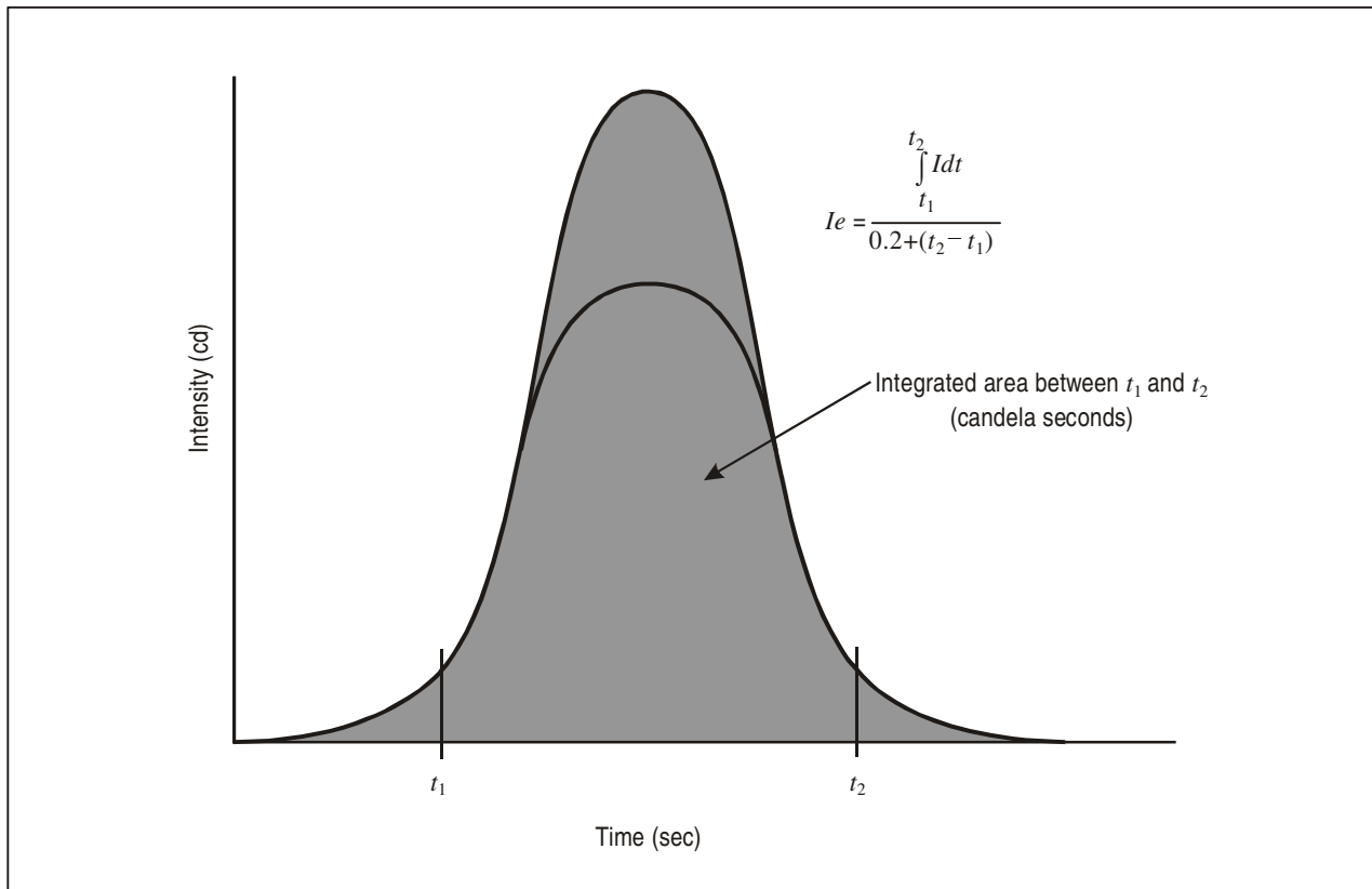
Figure 18-1. Typical flashing light that rises and falls gradually
