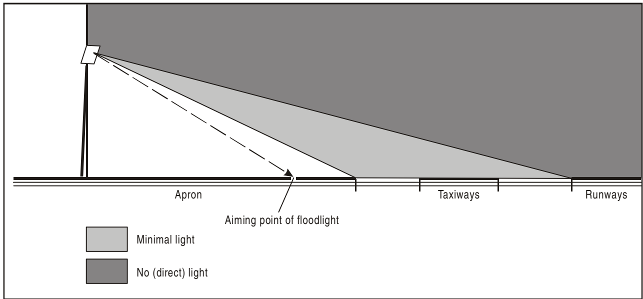
Figure 13-5. Aiming to avoid glare
