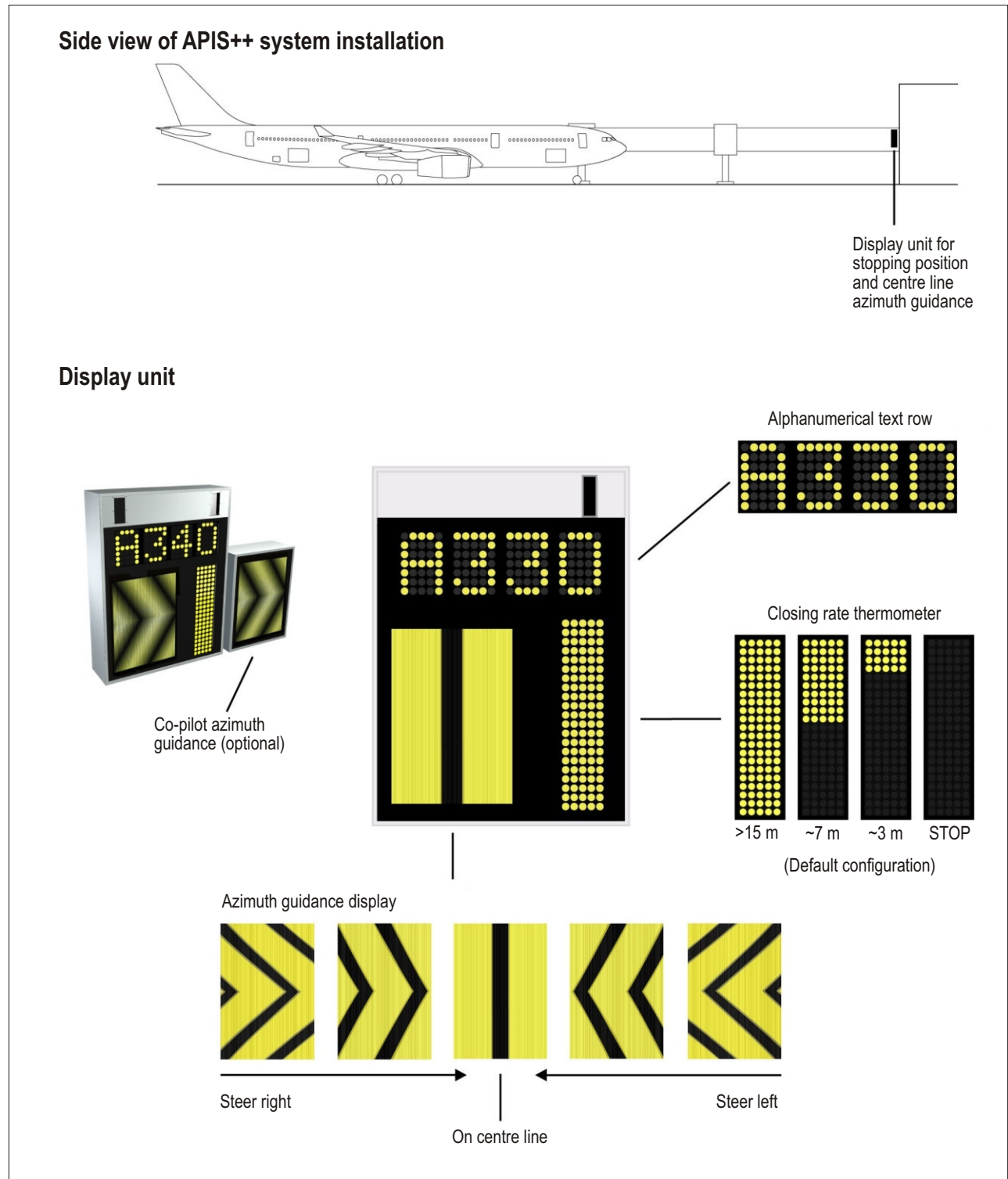
Figure 12-2. A visual docking guidance system using a graphical display (Moiré technique) to provide azimuth guidance and a laser radar to provide distance-to-go and stopping position information
