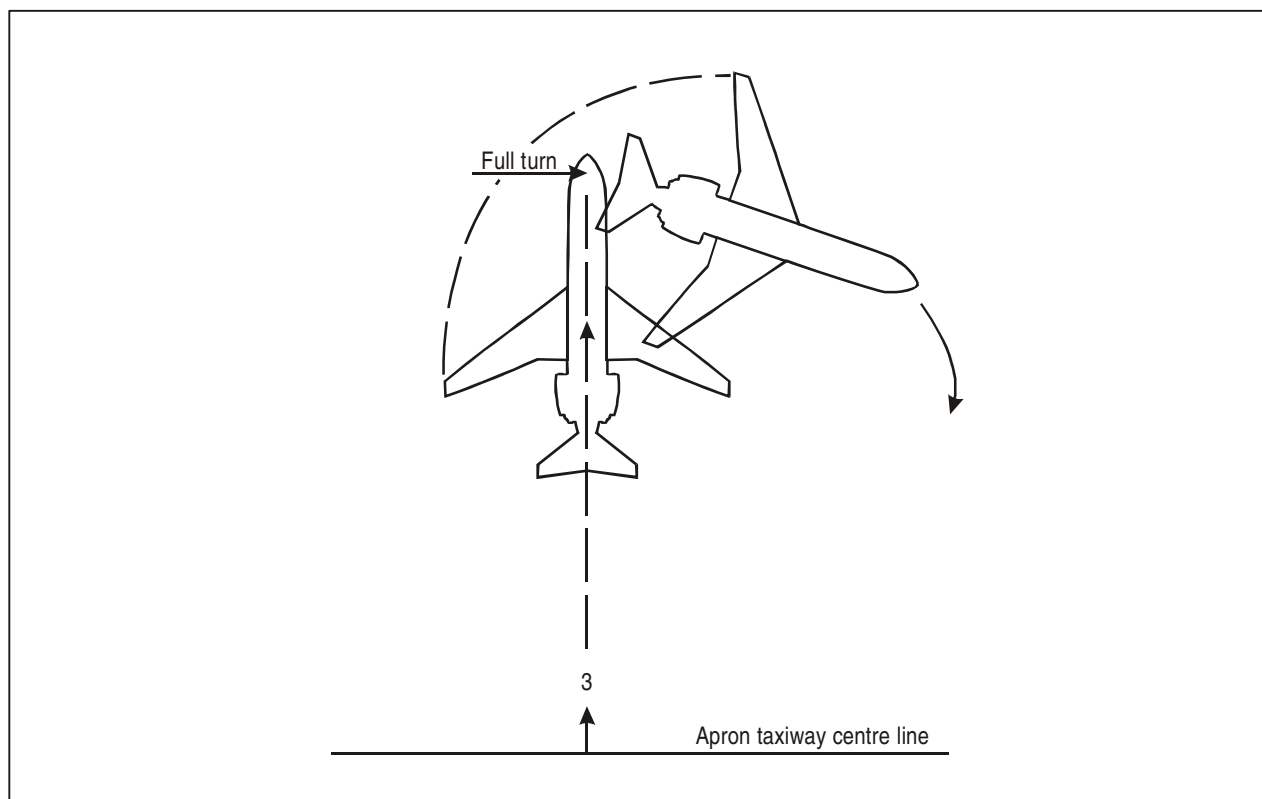
Figure 2-4. Straight lead-in line
