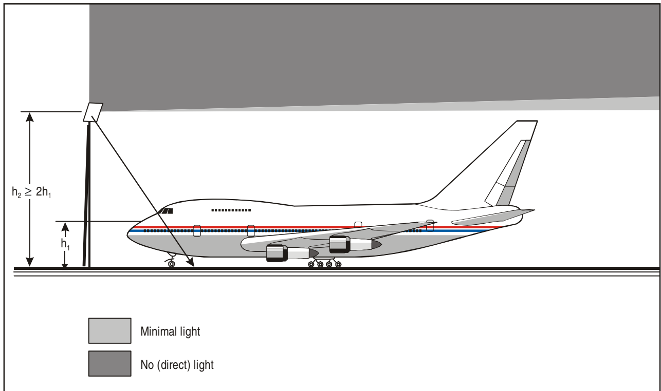
Figure 13-6. Mounting height to avoid glare
