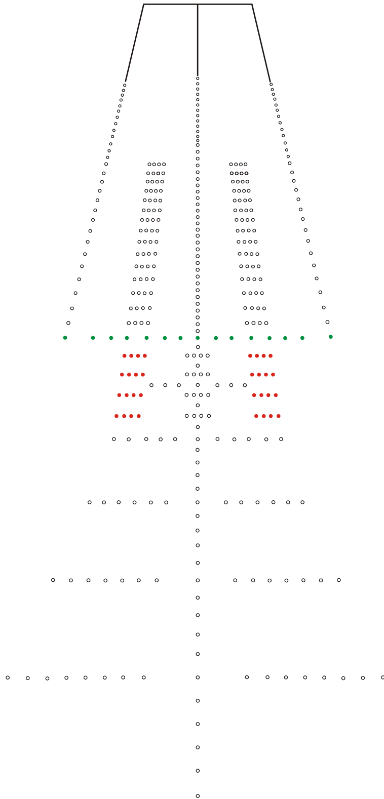
Figure 16-2. Approach and runway lighting, reduced pattern
