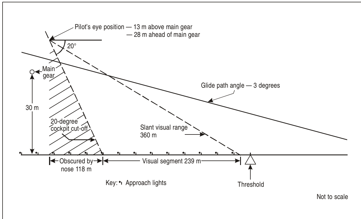
Figure 1-2. Visual segment from a large-bodied jet aircraft
