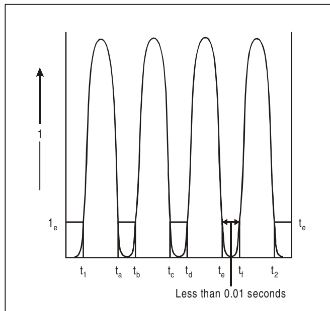
Figure 18-2. Flashing light producing very short flashes
