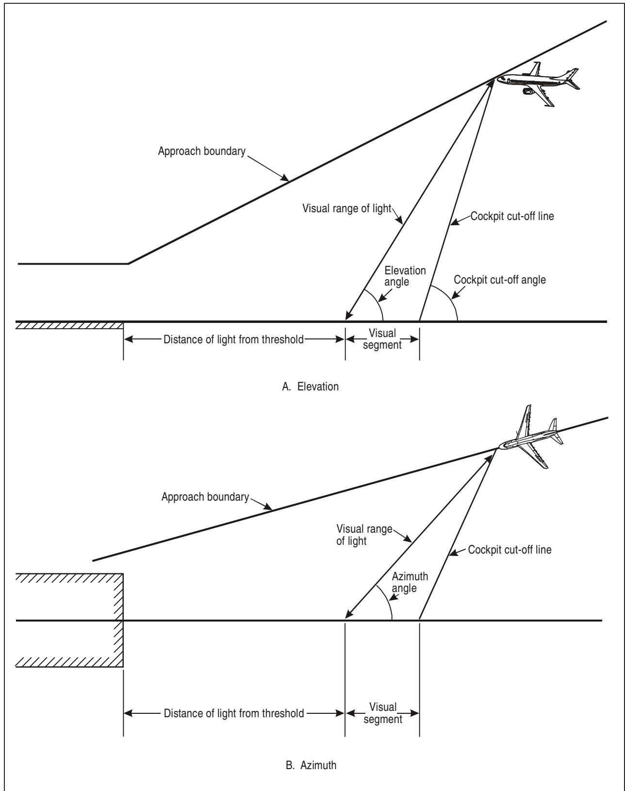
Figure 4-1. Visual segment geometry
