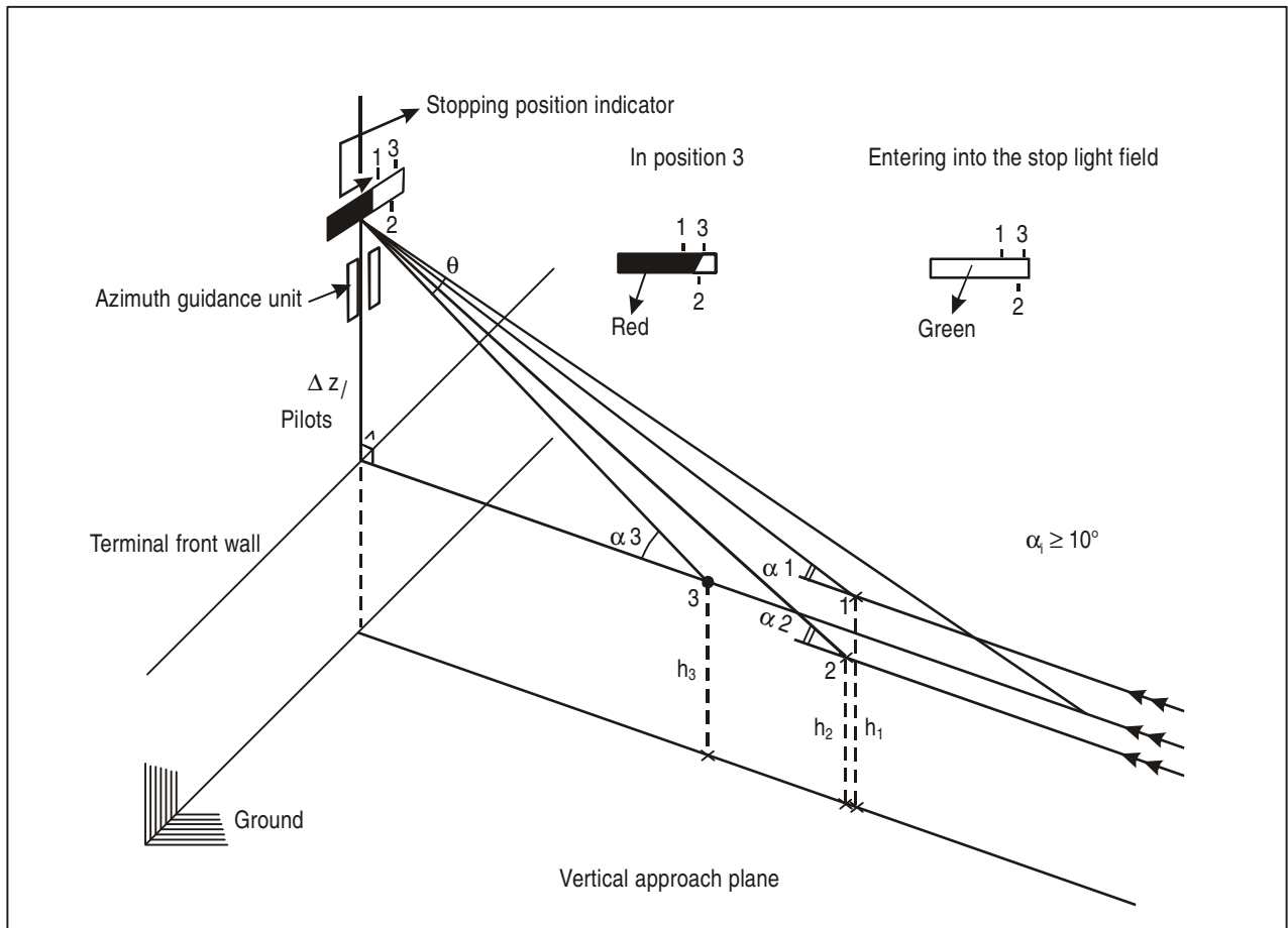
Figure 12-4. The stopping position indicator of a visual docking guidance system using lights
