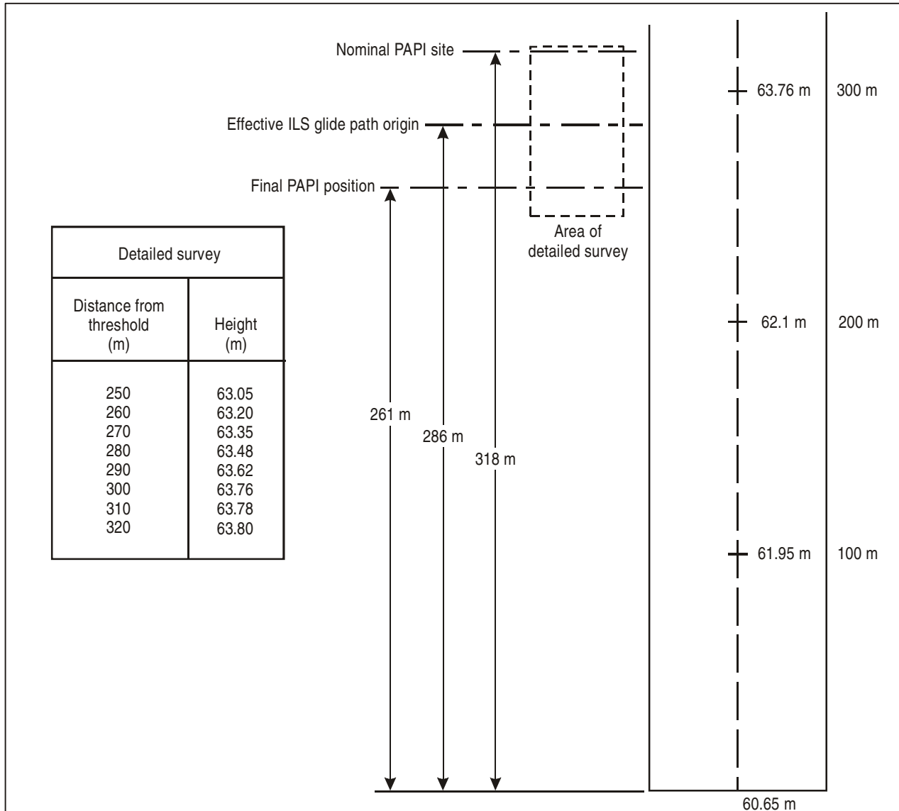
Figure 8-12. Survey data
