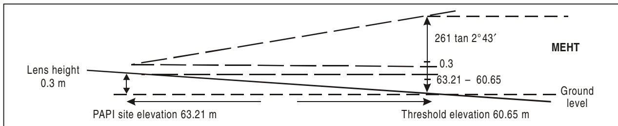
Figure 8-13. MEHT back-check
