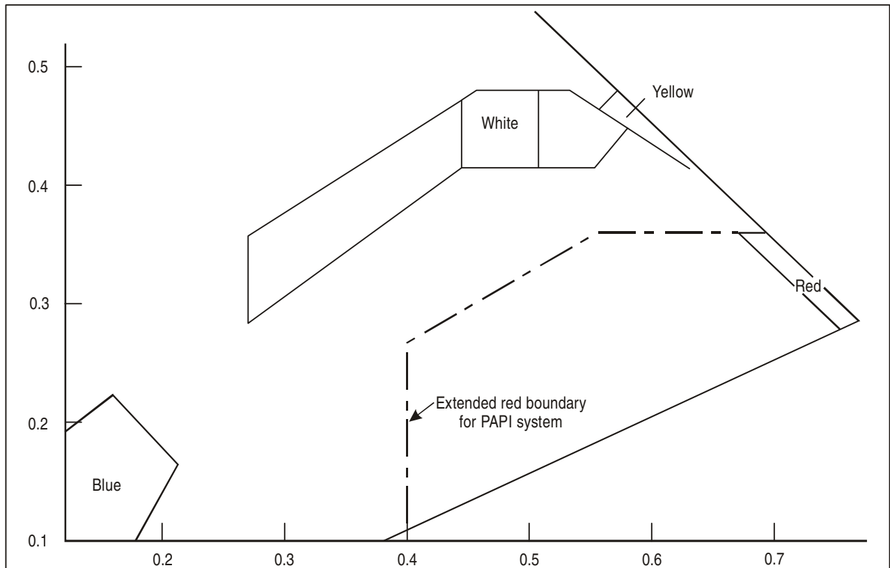
Figure 8-11. Suggested practical boundary for red PAPI
