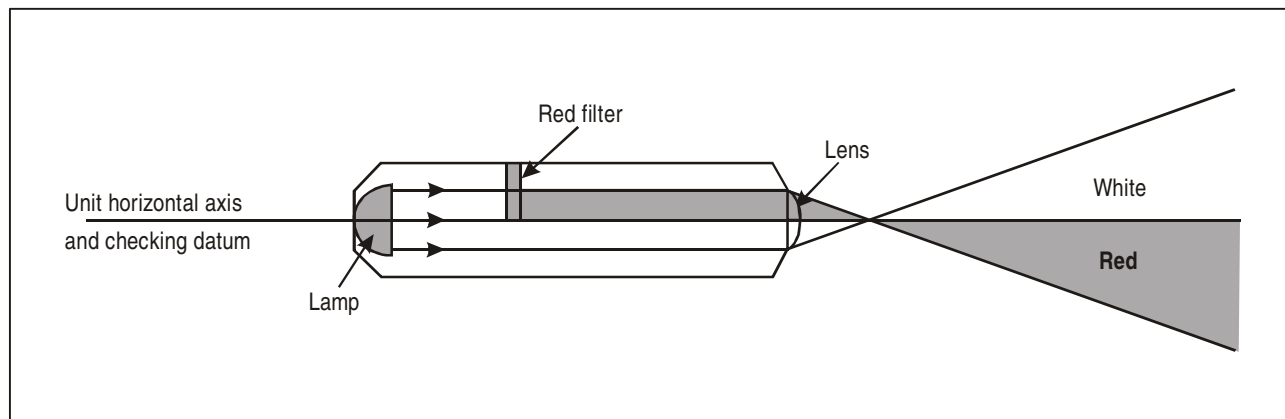
Figure 8-9. PAPI light unit
